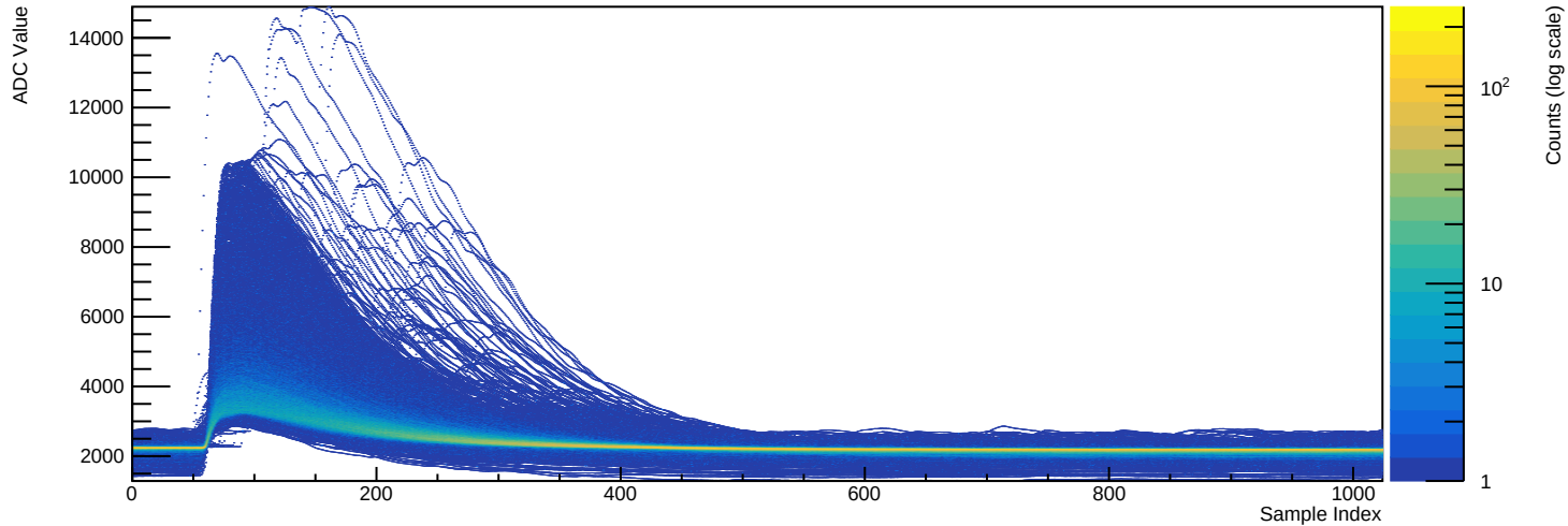
Run 039501 - Channel 2080 (n=8255 waveforms)
