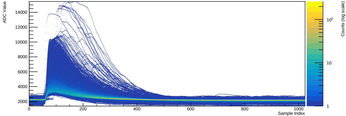
Run 039502 - Channel 2080 (n=8846 waveforms)
