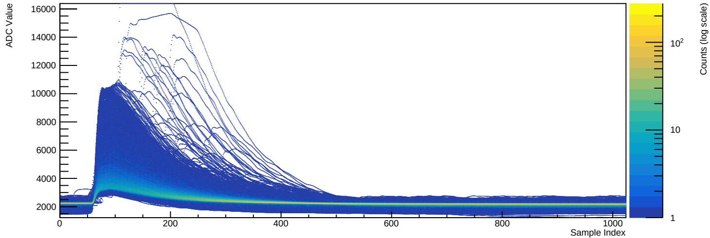
Run 039503 - Channel 2080 (n=9674 waveforms)
