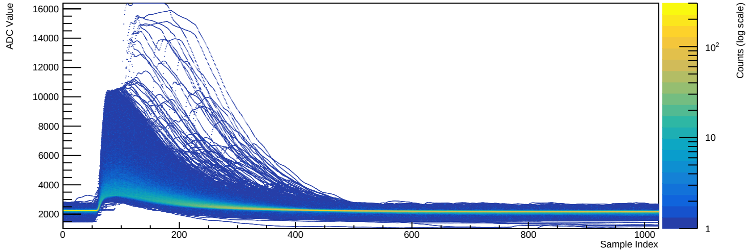
Run 039504 - Channel 2080 (n=10708 waveforms)
