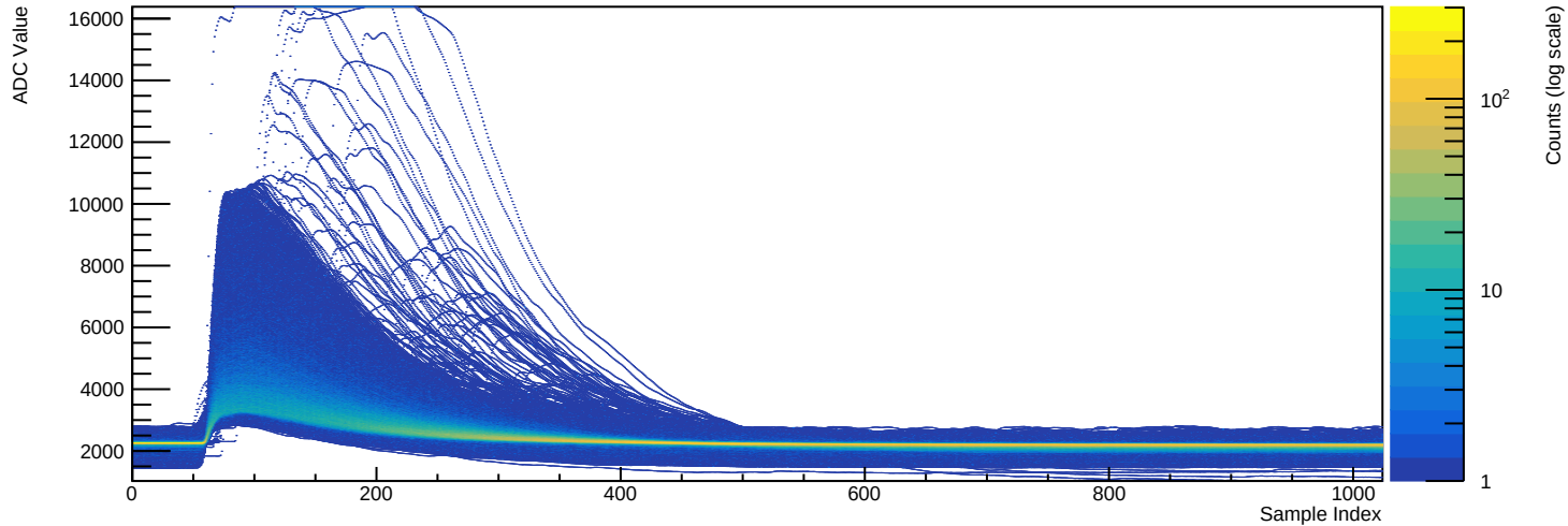
Run 039506 - Channel 2080 (n=11696 waveforms)
