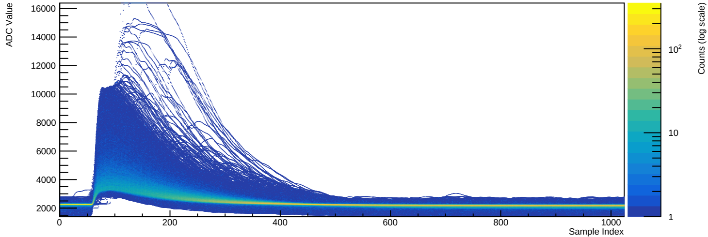
Run 039507 - Channel 2080 (n=12984 waveforms)
