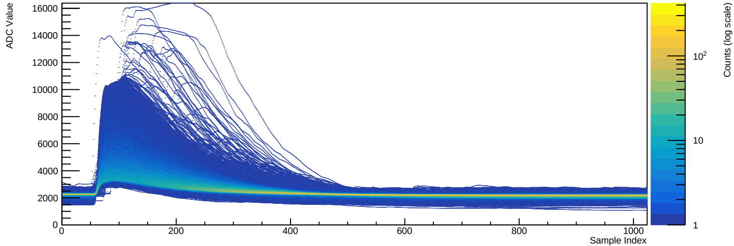
Run 039510 - Channel 2080 (n=16364 waveforms)
