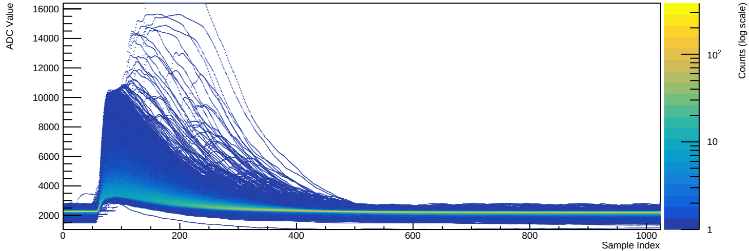
Run 039516 - Channel 2080 (n=11876 waveforms)
