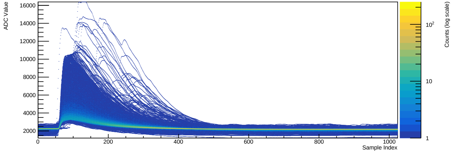
Run 039500 - Channel 2081 (n=7437 waveforms)
