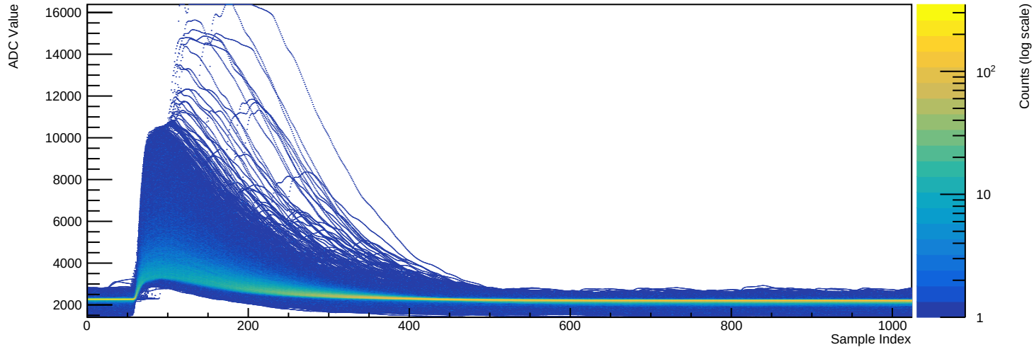
Run 039507 - Channel 2081 (n=12589 waveforms)
