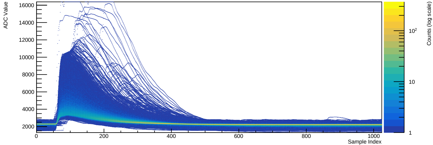
Run 039516 - Channel 2081 (n=11579 waveforms)
