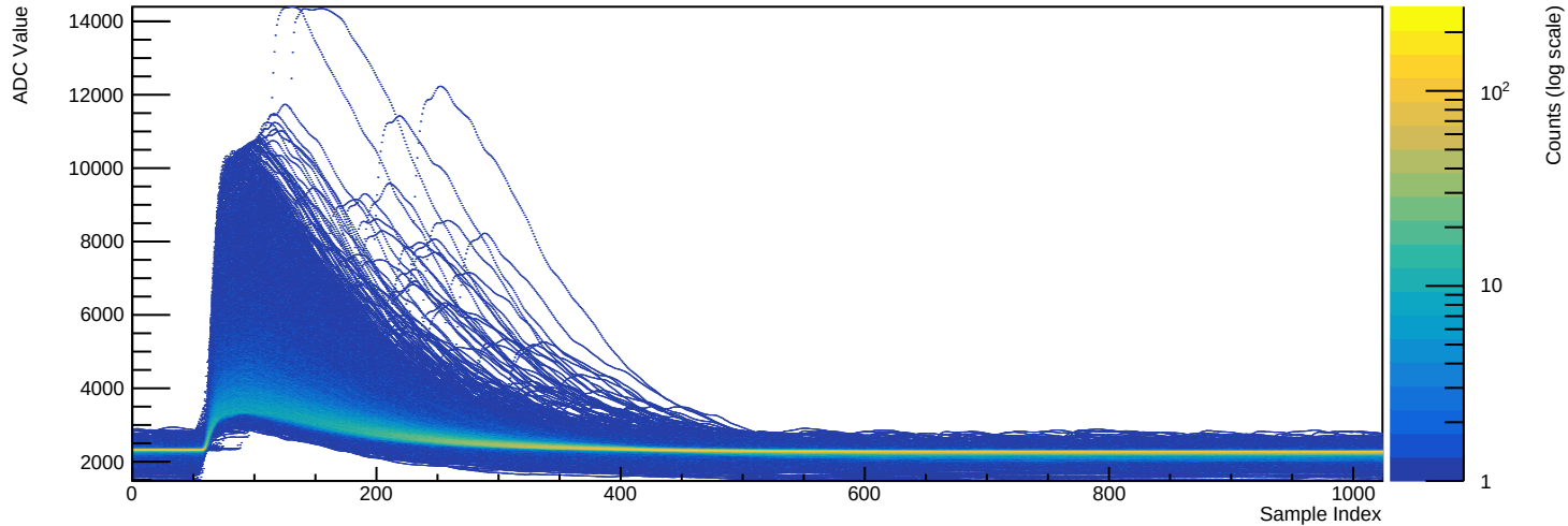
Run 039523 - Channel 2081 (n=8812 waveforms)
