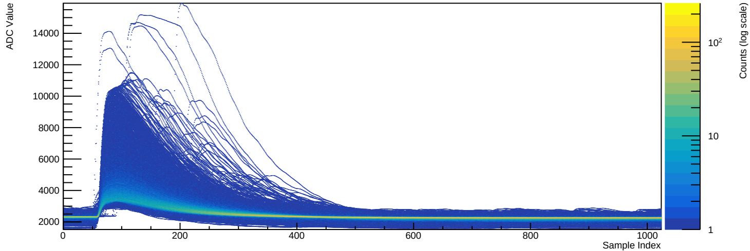
Run 039525 - Channel 2081 (n=8328 waveforms)
