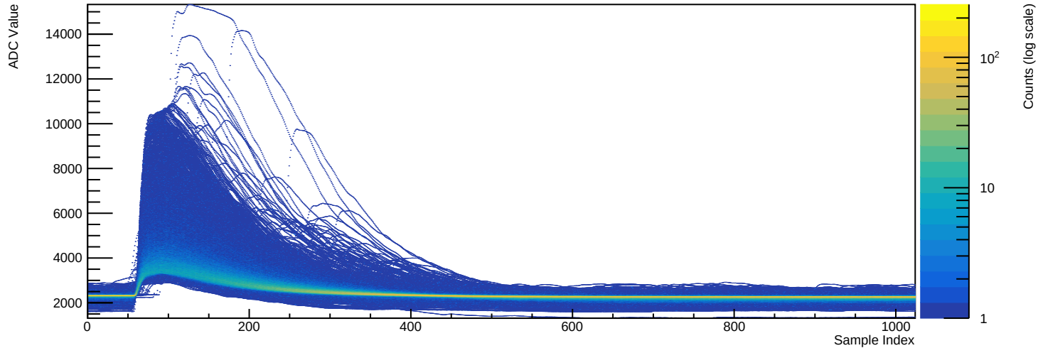
Run 039526 - Channel 2081 (n=7949 waveforms)
