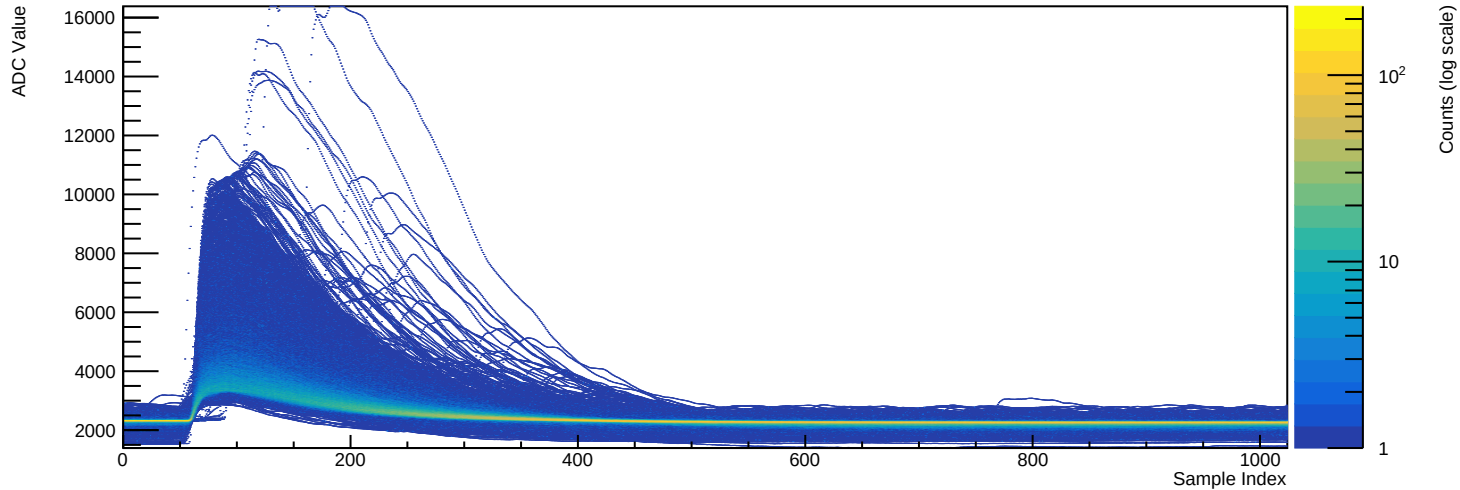
Run 039527 - Channel 2081 (n=7847 waveforms)
