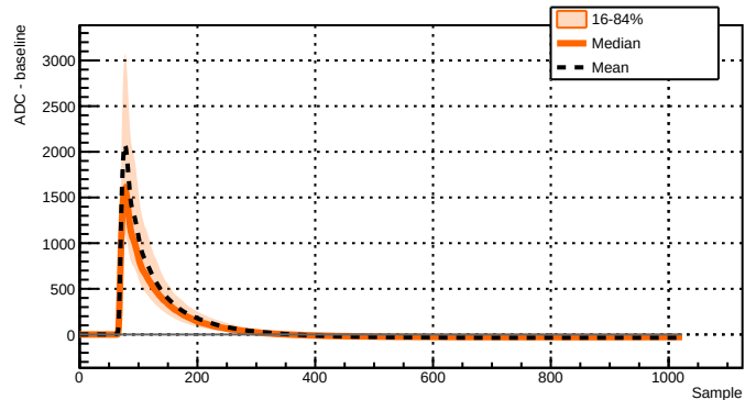
Run 039500 - Channel 2071 - 1129 waveforms
