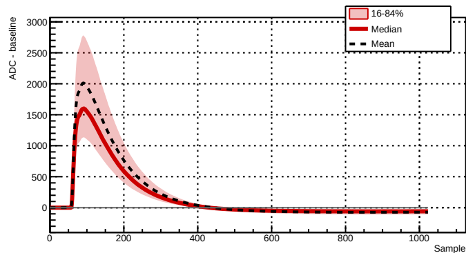
Run 039502 - Channel 2081 - 8497 waveforms
