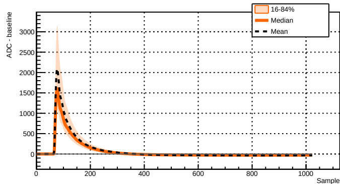
Run 039502 - Channel 2071 - 1326 waveforms
