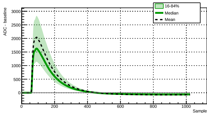
Run 039502 - Channel 2080 - 8846 waveforms
