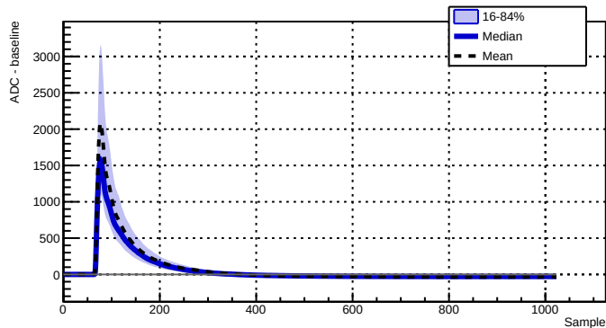
Run 039502 - Channel 2070 - 1415 waveforms
