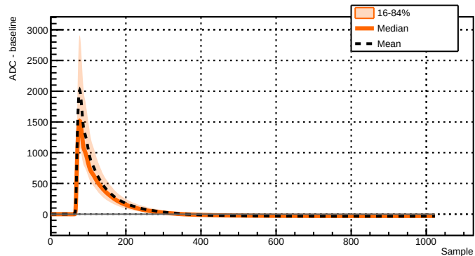
Run 039503 - Channel 2071 - 1462 waveforms
