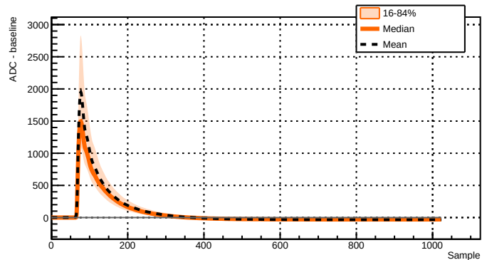
Run 039507 - Channel 2071 - 2069 waveforms
