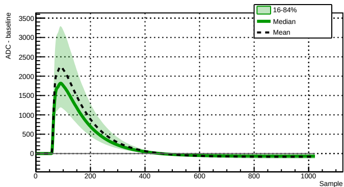
Run 039507 - Channel 2080 - 12984 waveforms
