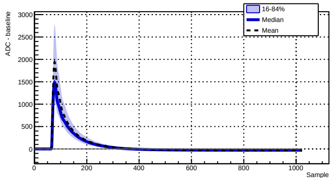
Run 039507 - Channel 2070 - 2196 waveforms
