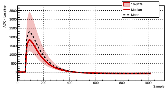
Run 039514 - Channel 2081 - 13311 waveforms
