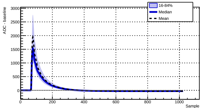
Run 039514 - Channel 2070 - 2601 waveforms
