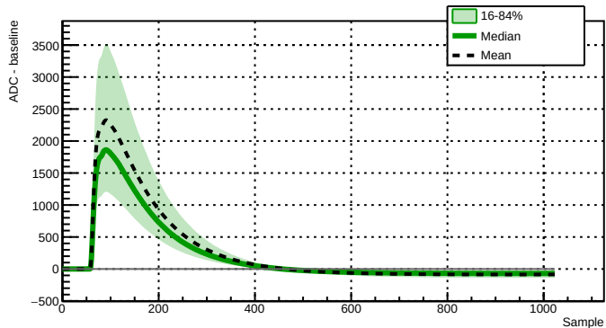
Run 039514 - Channel 2080 - 13625 waveforms
