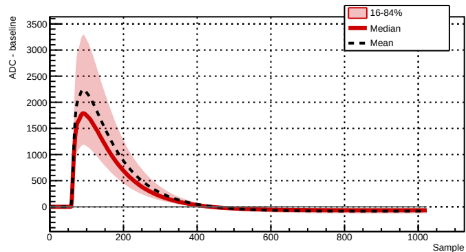
Run 039515 - Channel 2081 - 12182 waveforms
