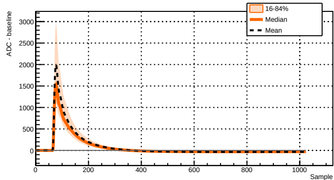
Run 039515 - Channel 2071 - 2131 waveforms
