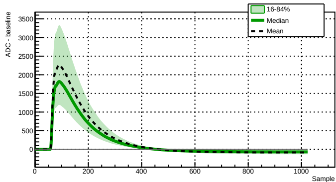
Run 039515 - Channel 2080 - 12553 waveforms
