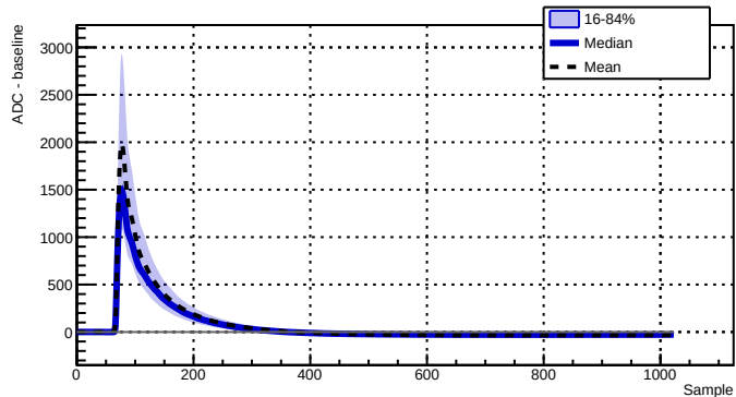
Run 039515 - Channel 2070 - 2272 waveforms
