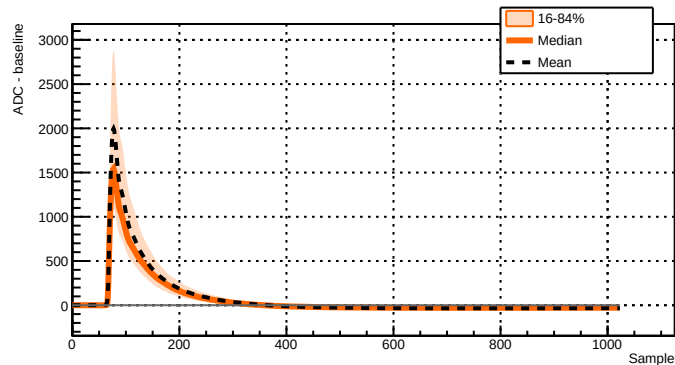
Run 039517 - Channel 2071 - 1856 waveforms
