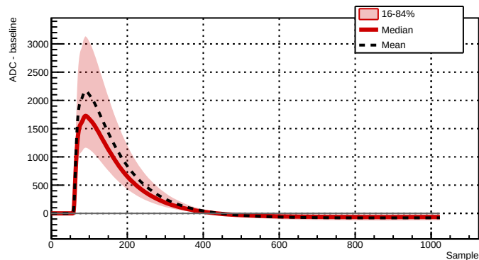
Run 039517 - Channel 2081 - 11335 waveforms
