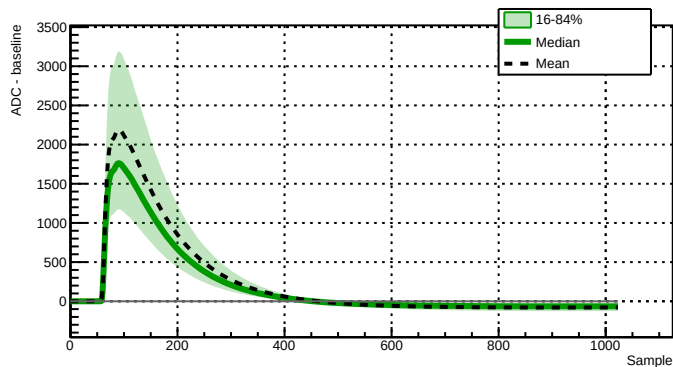
Run 039517 - Channel 2080 - 11634 waveforms
