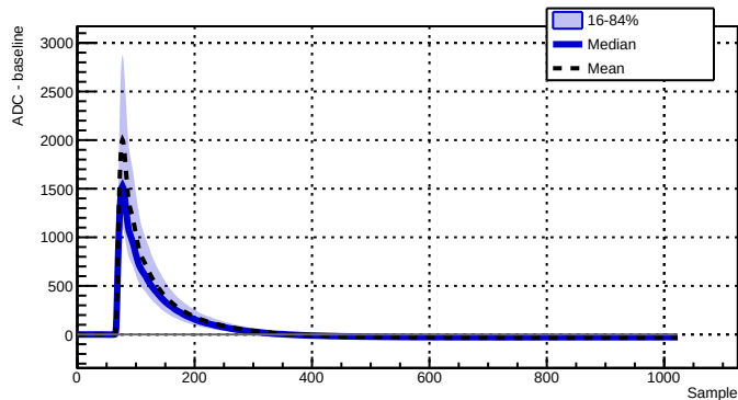
Run 039517 - Channel 2070 - 1948 waveforms
