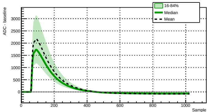
Run 039518 - Channel 2080 - 10999 waveforms
