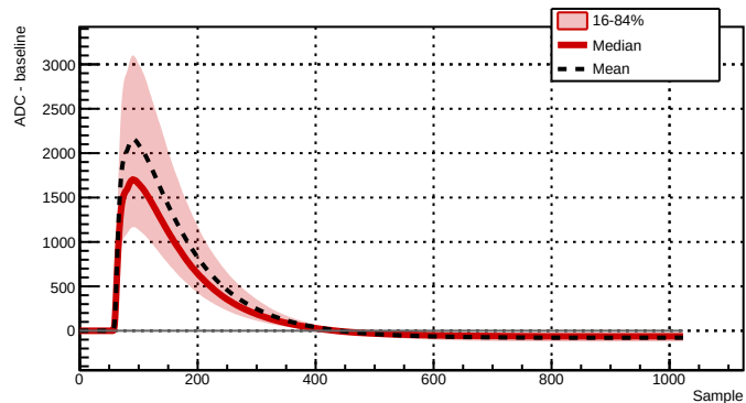
Run 039518 - Channel 2081 - 10631 waveforms
