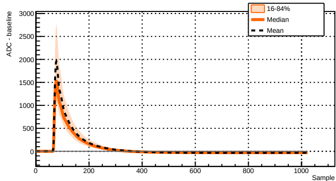
Run 039518 - Channel 2071 - 1749 waveforms
