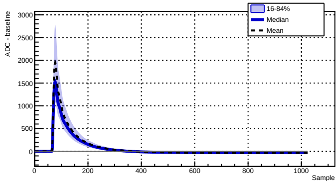
Run 039518 - Channel 2070 - 1843 waveforms
