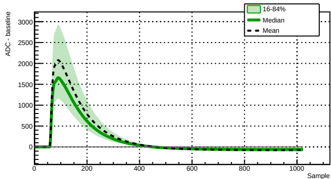
Run 039521 - Channel 2080 - 9867 waveforms
