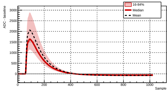
Run 039521 - Channel 2081 - 9497 waveforms
