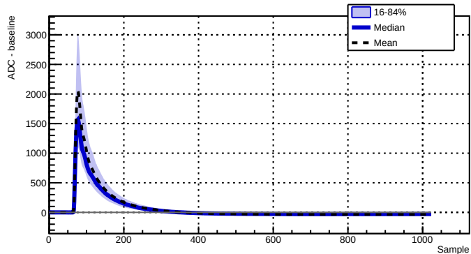
Run 039521 - Channel 2070 - 1538 waveforms
