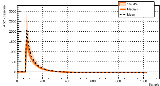
Run 039521 - Channel 2071 - 1473 waveforms
