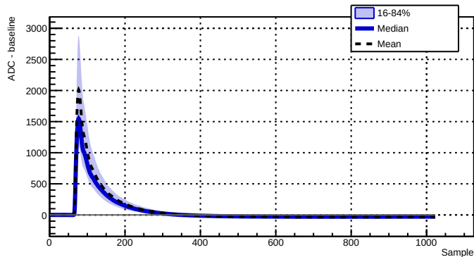
Run 039523 - Channel 2070 - 1412 waveforms
