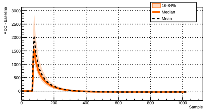
Run 039523 - Channel 2071 - 1336 waveforms
