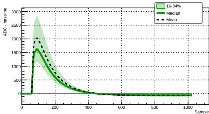
Run 039523 - Channel 2080 - 9111 waveforms
