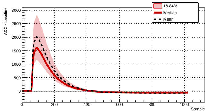
Run 039523 - Channel 2081 - 8812 waveforms
