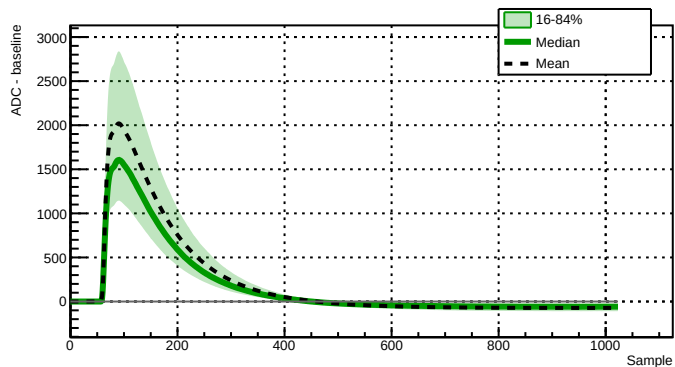
Run 039525 - Channel 2080 - 8608 waveforms
