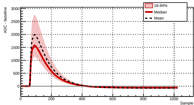
Run 039525 - Channel 2081 - 8328 waveforms
