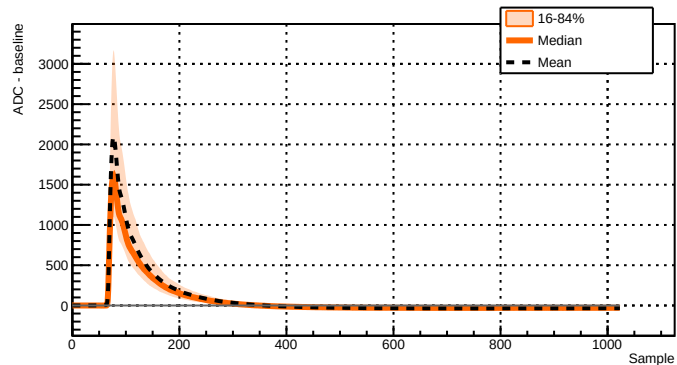
Run 039525 - Channel 2071 - 1249 waveforms
