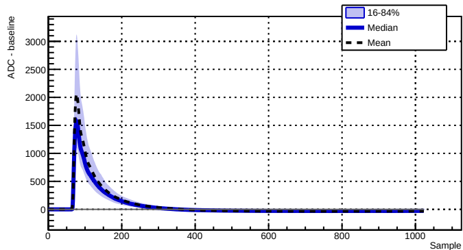
Run 039525 - Channel 2070 - 1344 waveforms
