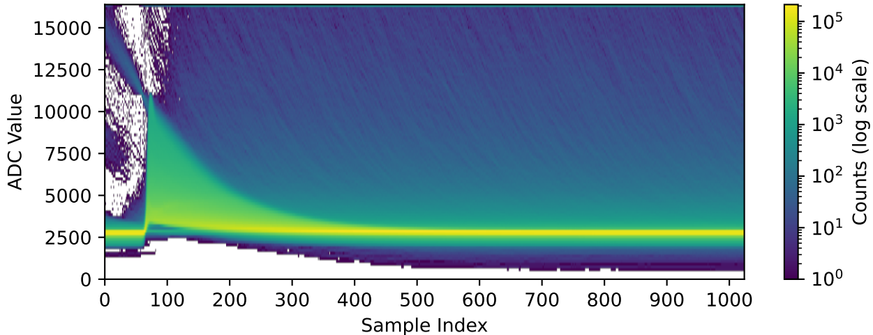
Channel 1010 (n=327515 waveforms)
