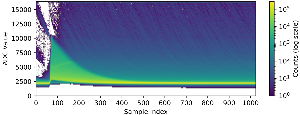
Channel 1020 (n=309647 waveforms)
