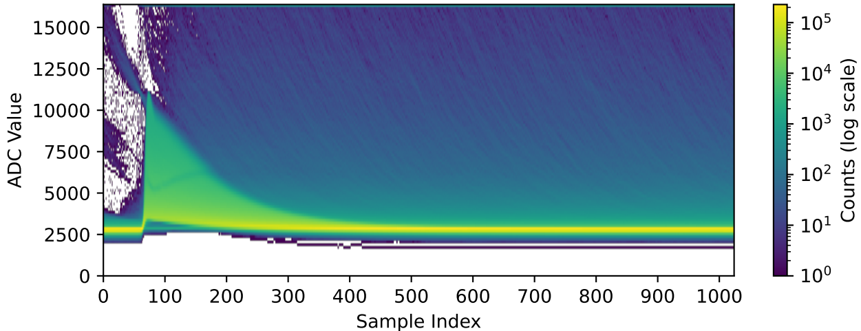
Channel 1040 (n=315748 waveforms)
