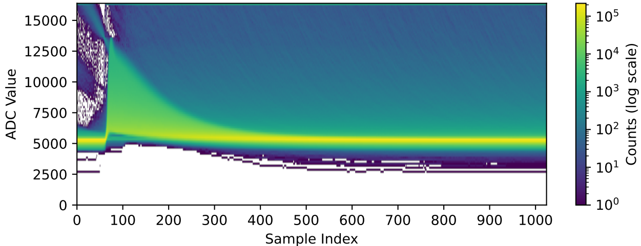
Channel 1051 (n=385208 waveforms)
