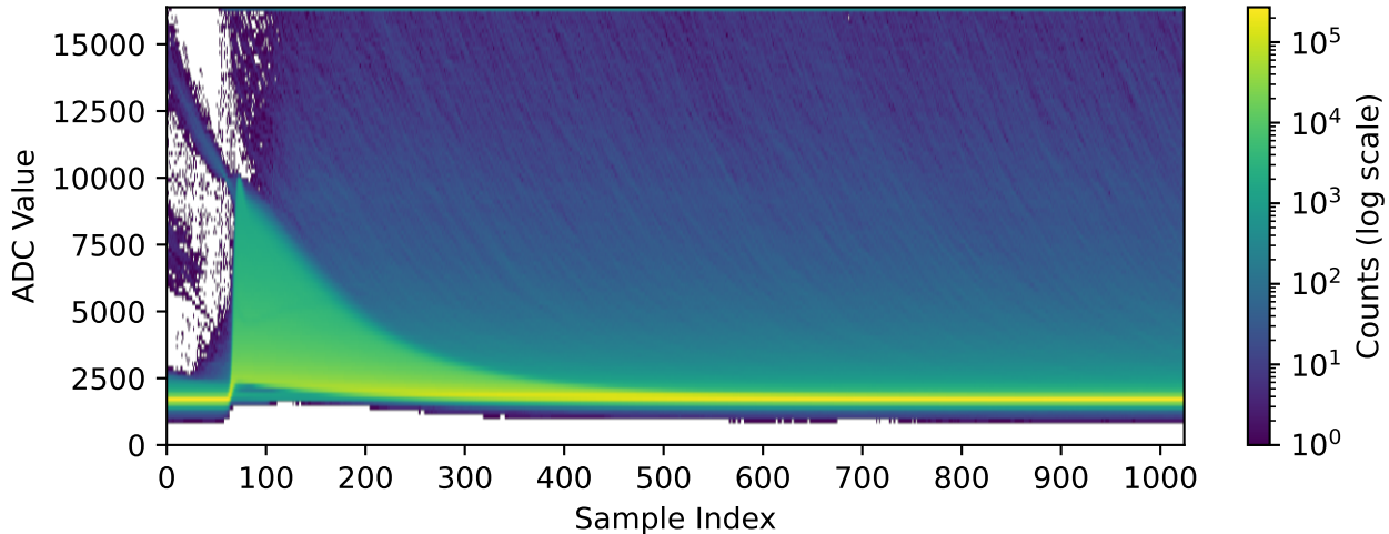
Channel 1060 (n=314532 waveforms)
