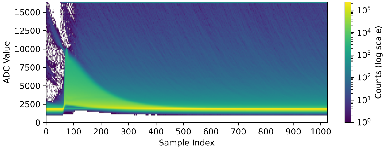
Channel 1061 (n=334828 waveforms)
