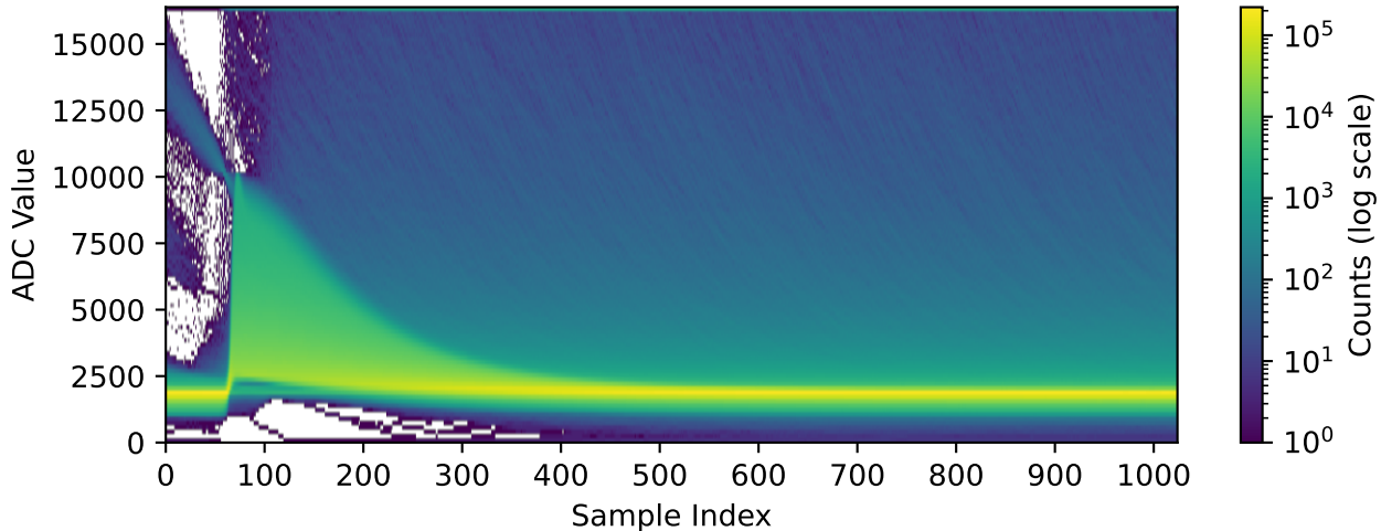
Channel 1070 (n=364147 waveforms)
