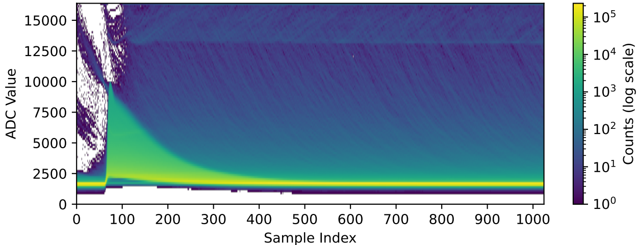
Channel 1081 (n=302198 waveforms)
