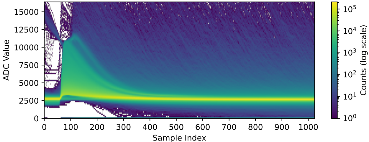
Channel 2040 (n=289756 waveforms)
