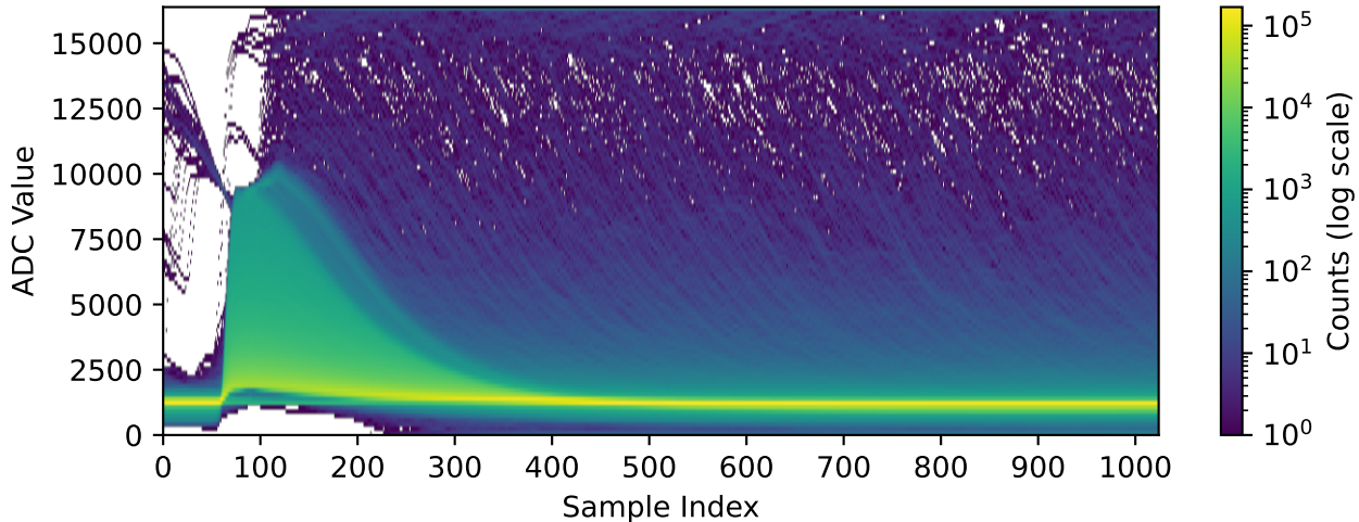
Channel 2051 (n=197727 waveforms)
