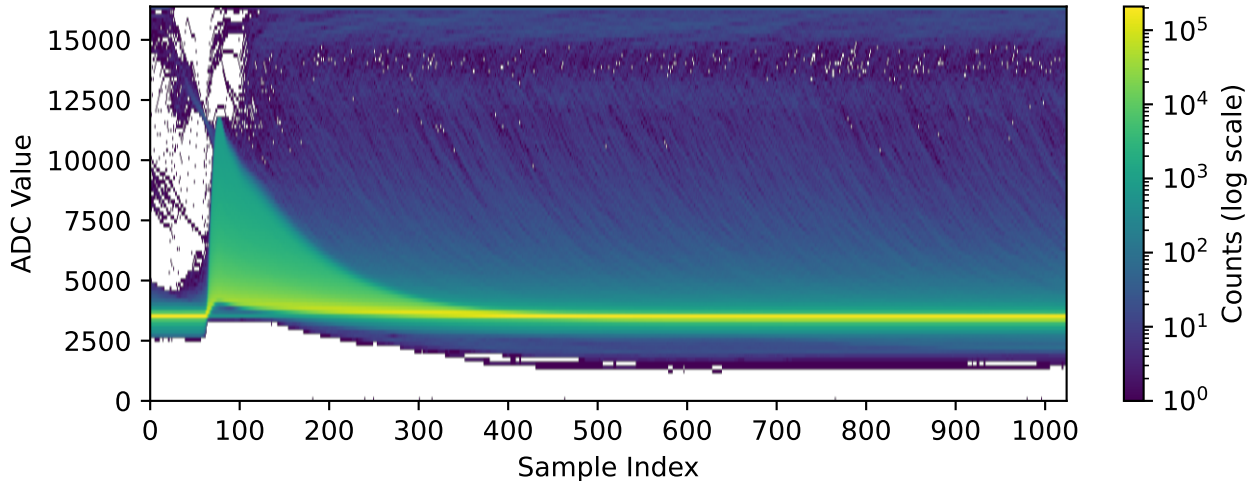
Channel 2060 (n=226425 waveforms)
