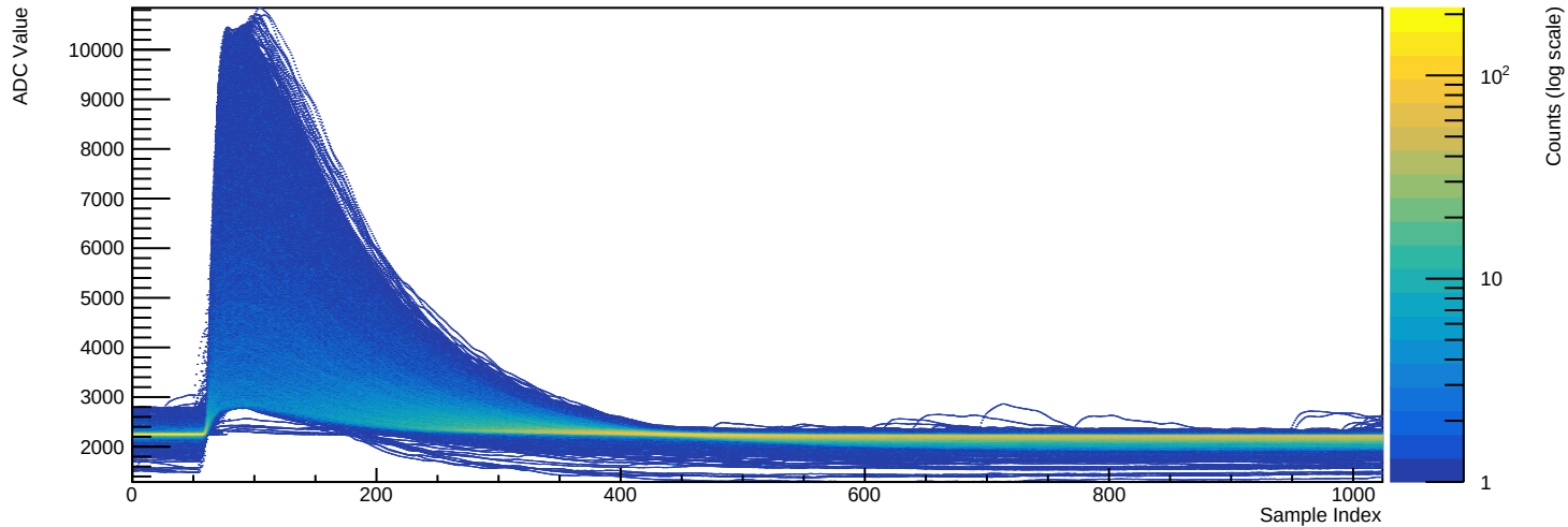
Run 039501 - Channel 2080 (n=7369 waveforms)
