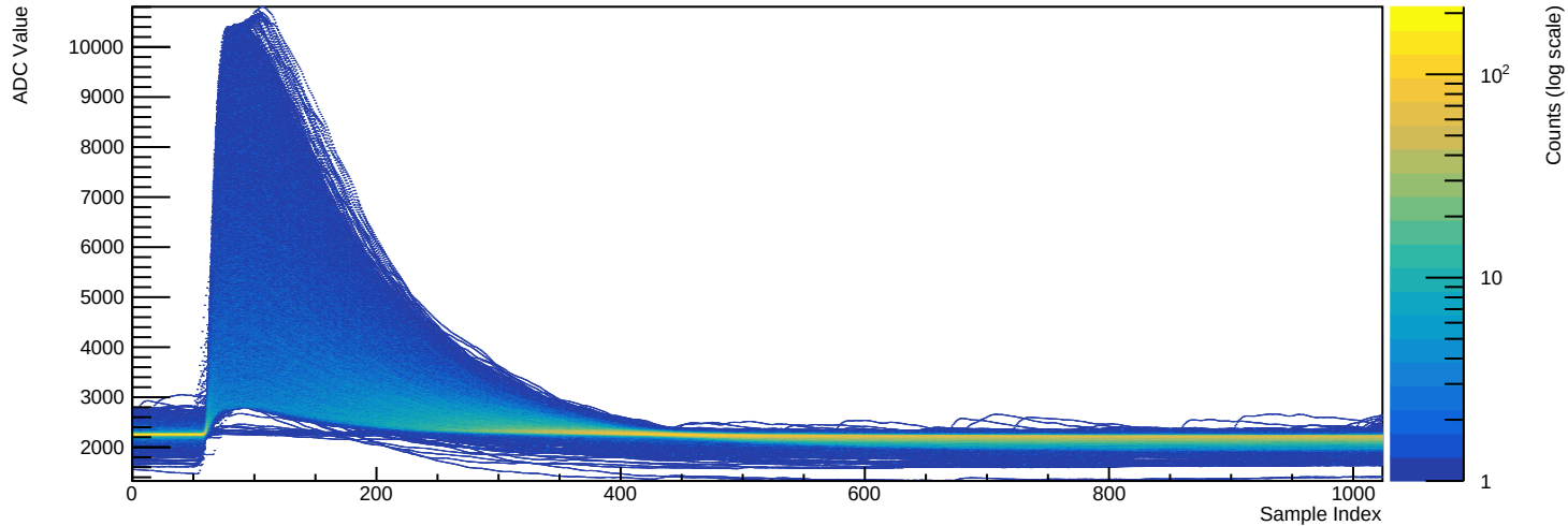
Run 039502 - Channel 2080 (n=7515 waveforms)
