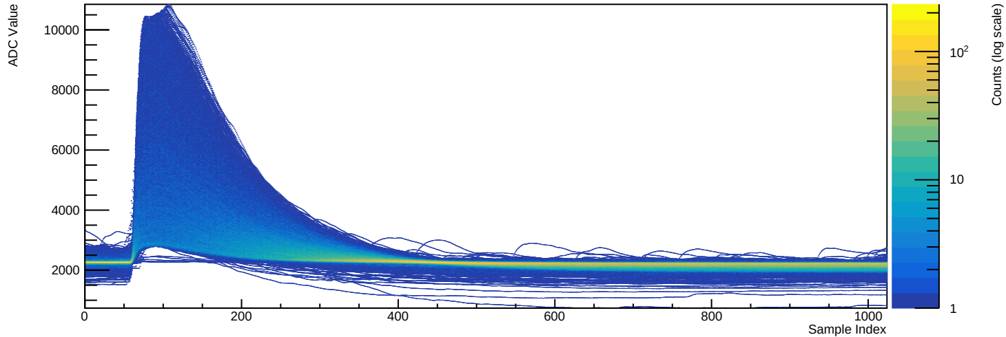
Run 039504 - Channel 2080 (n=8106 waveforms)
