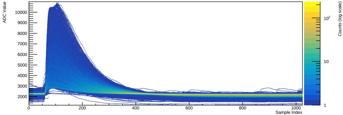
Run 039506 - Channel 2080 (n=8671 waveforms)
