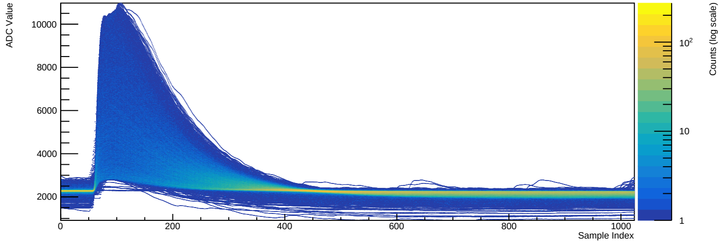
Run 039508 - Channel 2080 (n=9682 waveforms)
