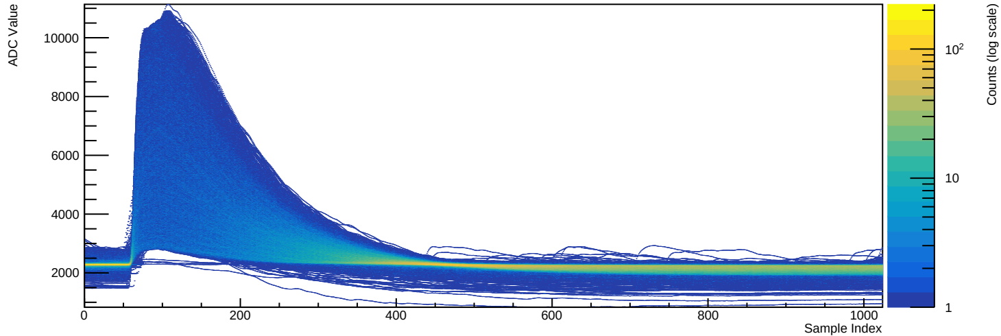
Run 039510 - Channel 2080 (n=8686 waveforms)
