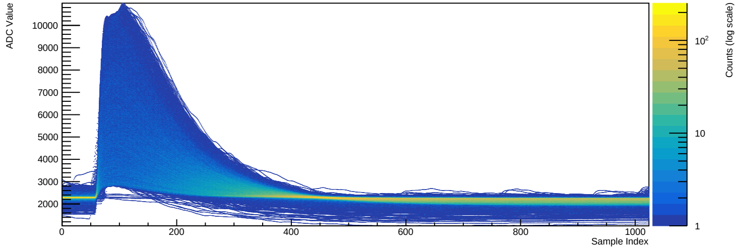
Run 039511 - Channel 2080 (n=10016 waveforms)
