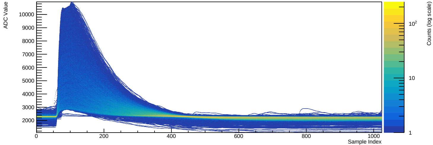
Run 039514 - Channel 2080 (n=9507 waveforms)
