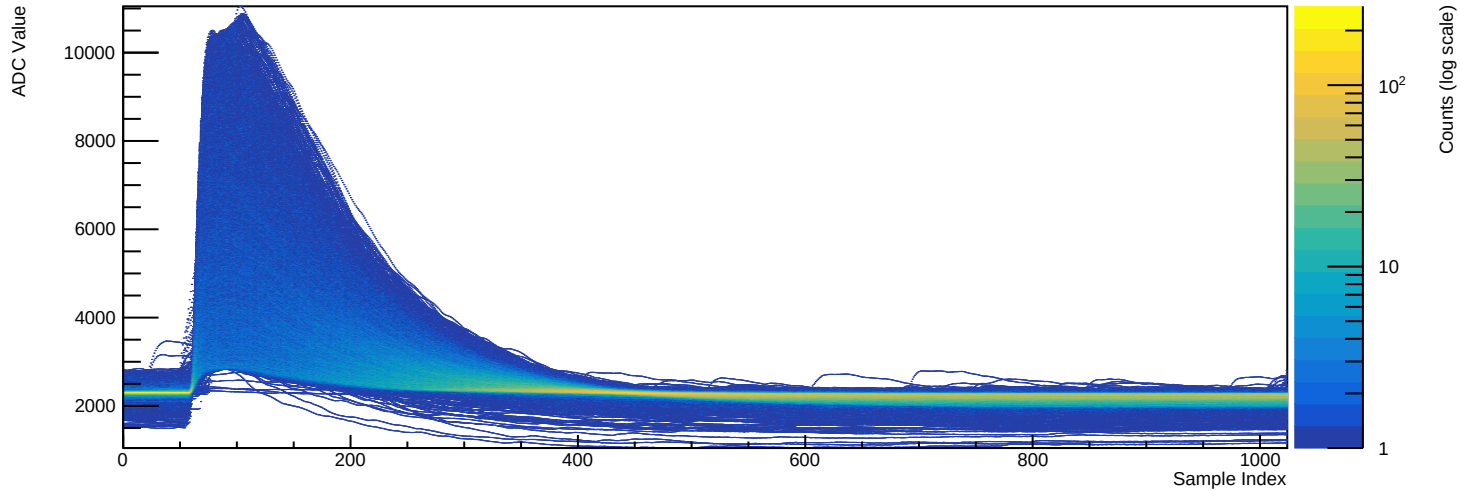
Run 039516 - Channel 2080 (n=8775 waveforms)
