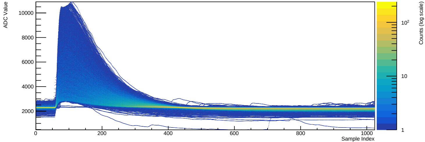
Run 039517 - Channel 2080 (n=8769 waveforms)
