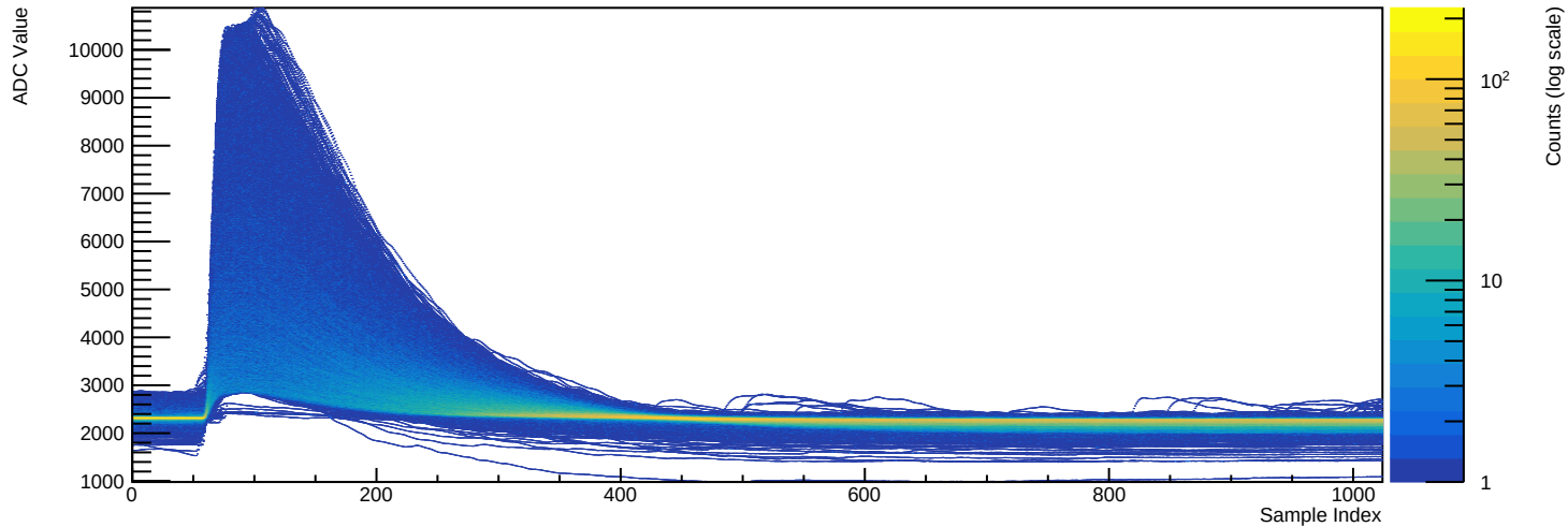
Run 039523 - Channel 2080 (n=7640 waveforms)
