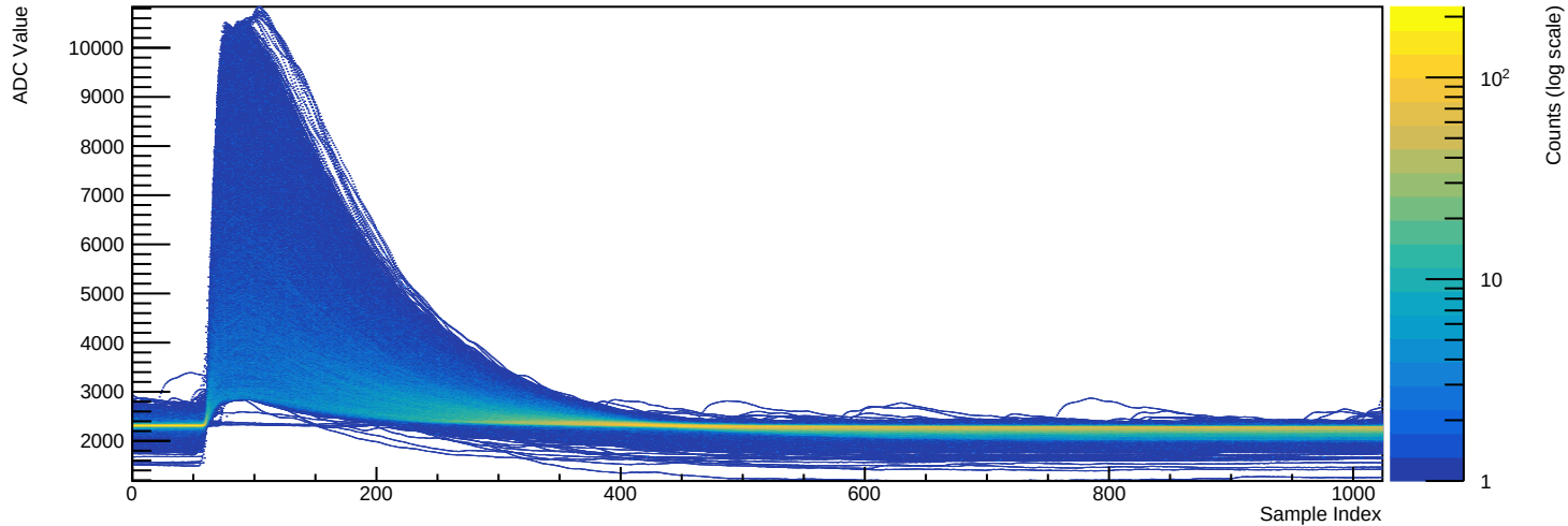
Run 039527 - Channel 2080 (n=7271 waveforms)
