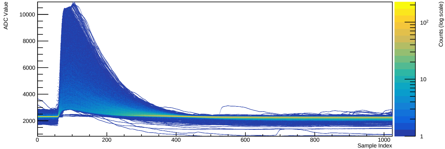
Run 039528 - Channel 2080 (n=7142 waveforms)
